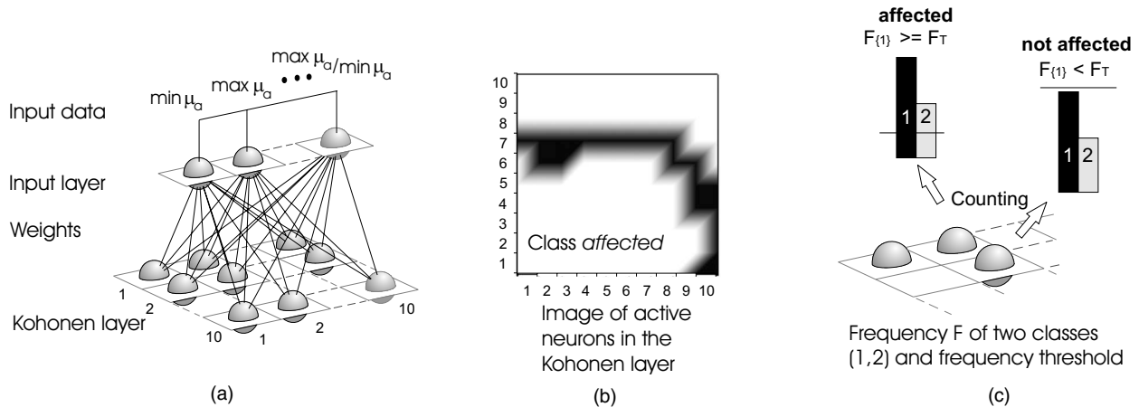
Fig. 2 Scheme for multiparameter classifications based on self-organizing maps (SOM): (a) Structure of a SOM neural network, (b) image of active neurons representing the class affected within the Kohonen layer after discrimination of the given input vectors, and (c) frequency determination and final classification of the classes affected (black) and not affected (gray). A frequency threshold F_T varying between 0 and 100% can be used to determine multiparameter ROC curves (Fig. 3).
